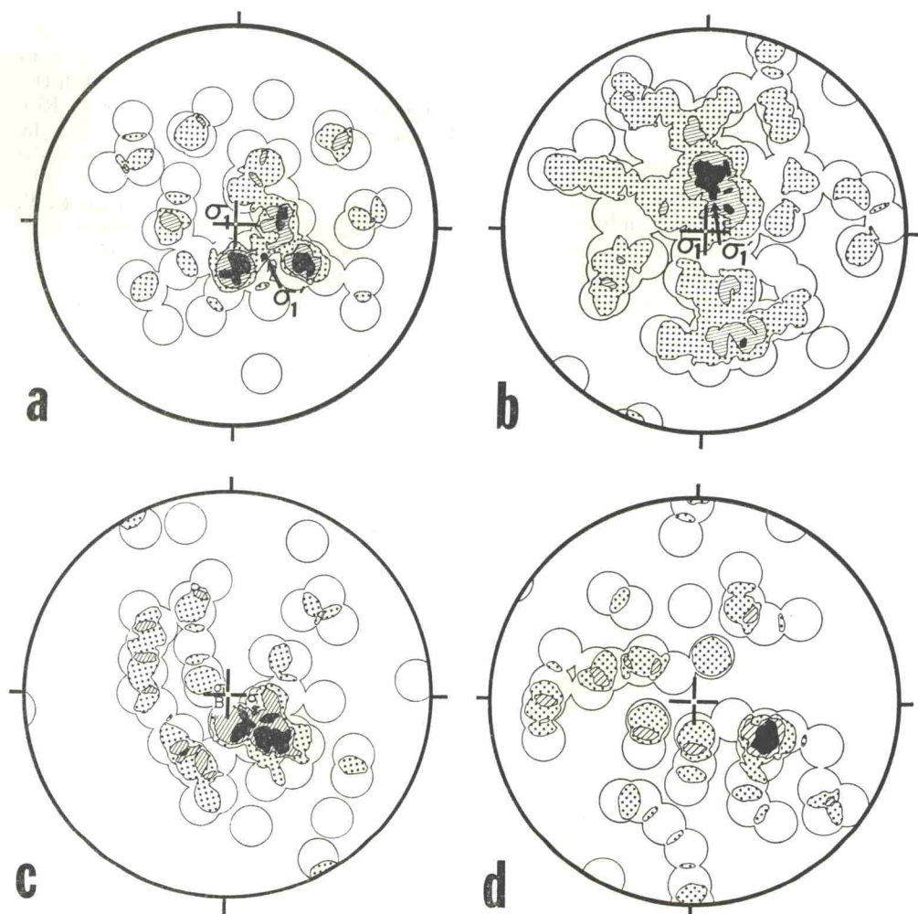
FIG. 16.—Diagrams illustrating orientation of compression axes derived from e_1 twin lamellae in specimens 762, 725, 778, and 780. Plane of each diagram is oriented normal to the long axis of the deformed cylinder, and \sigma_1 is at the center. a , specimen 762. Diagram of 50 compression axes. Contours: 2, 4, 6, and 8 per cent per 1 per cent area; 10 per cent maximum. Center of gravity ( \sigma'_1 ) is about 20° SE. of center. b , specimen 725. Composite diagram of 100 compression axes. Contours: 1, 2, 4, and 6 per cent per 1 per cent area; 10 per cent maximum. Center of gravity ( \sigma'_1 ) is about 10° N. of center. c , specimen 778. Diagram of 50 compression axes. Contours: 2, 4, 6, and 8 per cent per 1 per cent area; 10 per cent maximum. Center of gravity ( \sigma_1 ) is 10°–15° SE. of center. d , specimen 780. Composite diagram of 50 compression axes. Contours: 2, 4, 6, and 8 per cent per 1 per cent area; 12 per cent maximum. There is a general grouping of the axes about the center.
